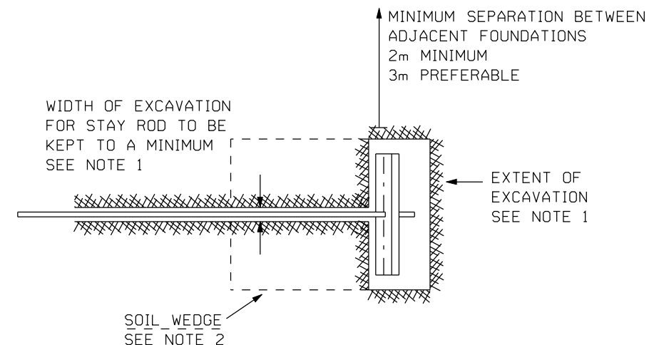
PLAN OF EXCAVATION LIMITS
